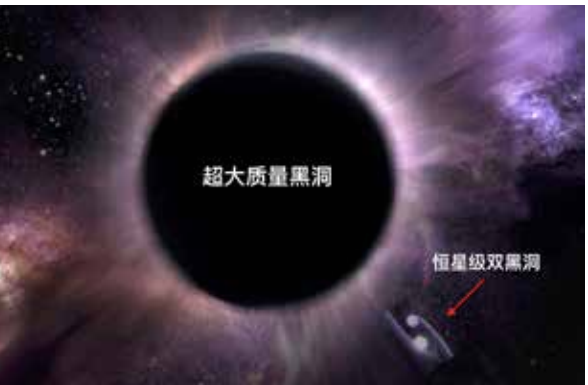
图一：双星极端质量比旋进系统想象图。 Figure 1: Illustration of a binary extreme-mass-ratio inspiral.
