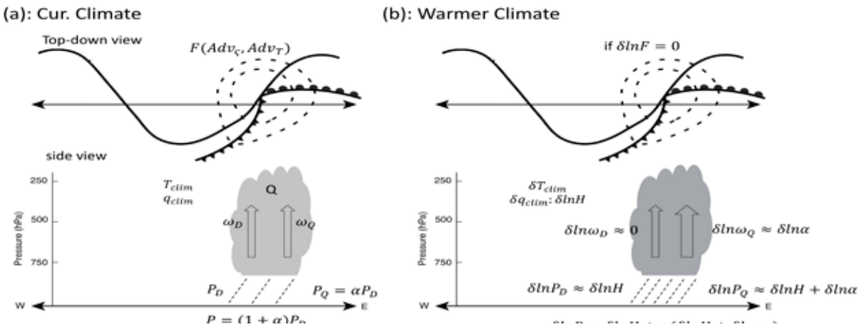
图 1：极端降雨在当前气候下的主要过程（a）和其对气候暖化的响应（b）的示意图。 Fig. A schematic of the scaling of precipitation extremes with temperature in a CQG system. (a) is under the current climate, and (b) is in a warmer climate.
