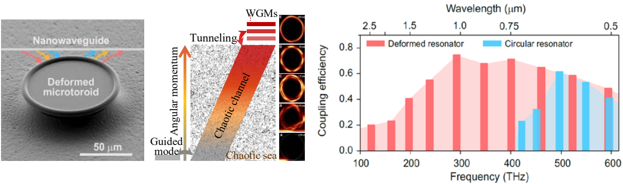
左：变形微腔扫描隧道显微镜图；中：混沌辅助动量转换耦合过程示意图；右：纳米光纤与变形 / 圆形微腔耦合效率仿真对比图 Left: SEM image of a deformed microresonator coupled with a nanowaveguide. Middle: Schematic for the chaos-assisted momentum-transformed coupling process. Inset: Short-time snapshots in 3D FDTD simulations of spatial intensity distribution. Right: 3D FDTD simulation showing coupling efficiencies of a deformed (red) and a circular (blue) microresonator coupled with a nanowaveguide.
