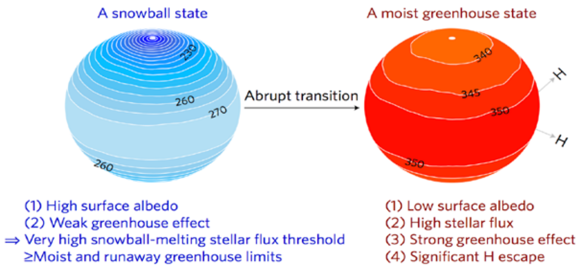
从冰雪世界到极端炎热世界的快速转换 Abrupt transition from a snowball state to an extremely hot climate state
