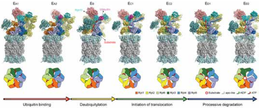
利用冷冻电镜解析的七个底物结合的人源 26S 蛋白酶体精细原子结构,揭示了从泛素识别、去泛素化反应、转运启动和持续降价的核心功能动态过程。 Seven cryo-EM structures at atomic-level resolution revealed the inner working of human proteasome and its dynamic substrate-processing steps of ubiquitin recognition, deubiquitylation, translocation initiation and processive substrate degradation. Credit: Shuwen Zhang and Youdong Mao.
